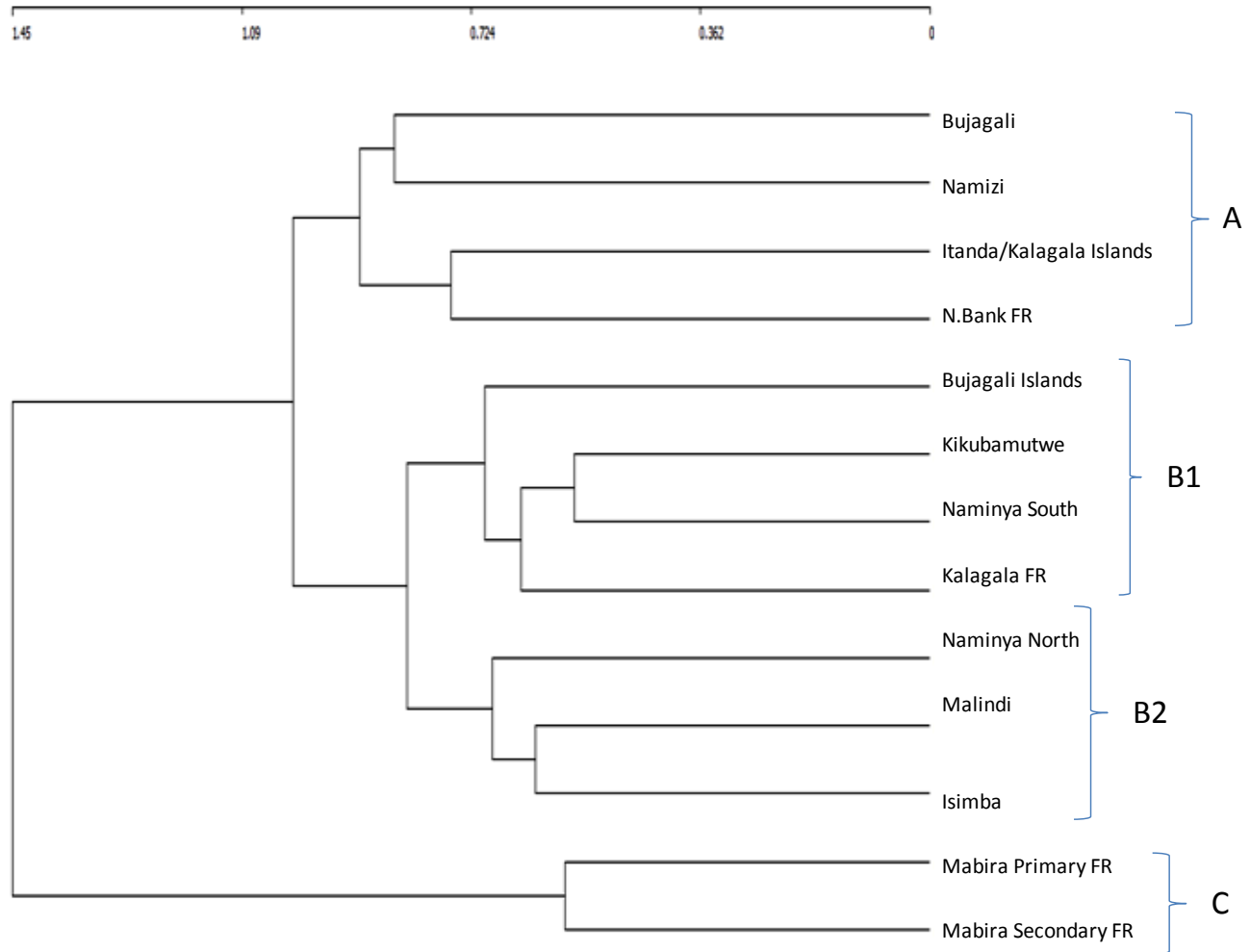
Figure 2: A Dendrogram from the Cluster analysis of 13 sites of the project area based upon the presence or absence of 451 plant species. Site groupings (A, B & C) were done with ANOSIM (Analysis of similarity) and SIMPER (Similarity percentage).
