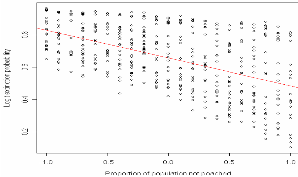
Figure 8b: Plot of logit extinction probability against standardized proportion of population not poached, following sensitivity analysis. Linear fit gives adjusted r^2 = 0.27 .
