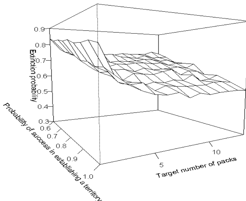
Figure 12: Plot of extinction probability against target number of packs, with all other parameters fixed but showing the effect of uncertainty in the value for probability of success in establishing territory.
