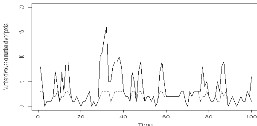
Figure 7: Example plot of wolf population and number of packs, in solid and dashed lines respectively, against time in years, under the present management regime. In this particular run, there were 73 years in which no breeding packs existed in Norway (i.e. extinction probability = 73%).
