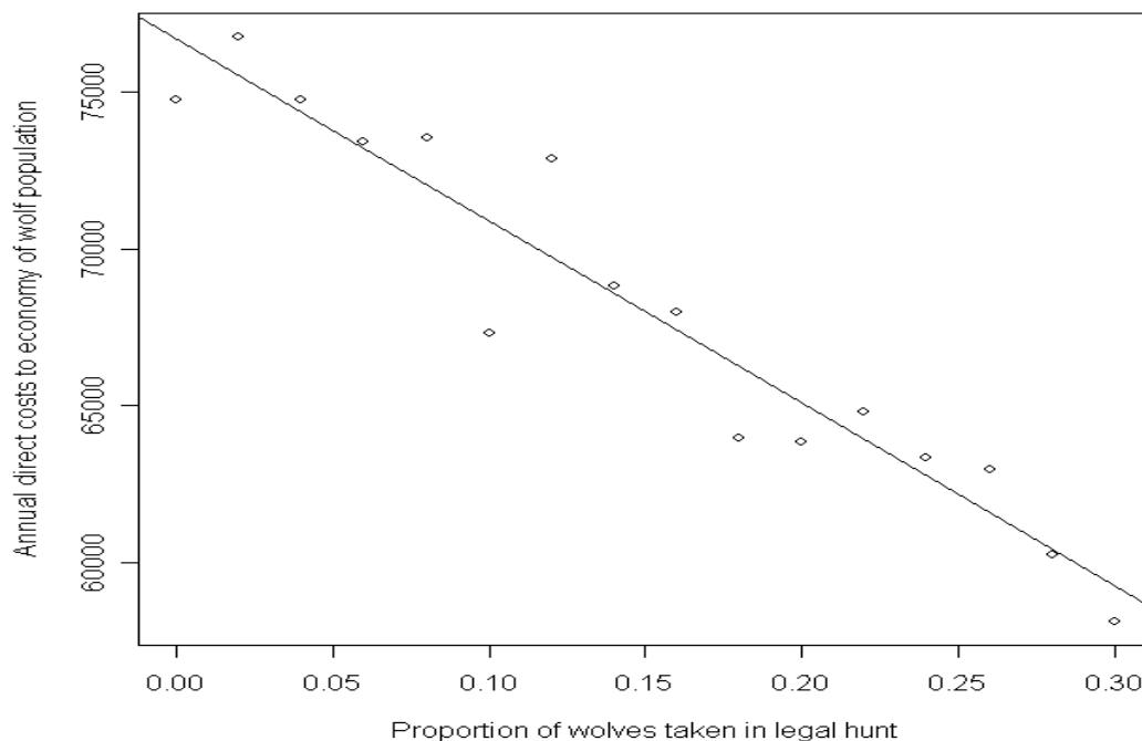
Figure 18: Plot of direct costs against proportion of wolves taken in an adaptive legal hunt, with a threshold population set at 15 individuals. Straight line fit gives adjusted r^2 = 0.9 .
