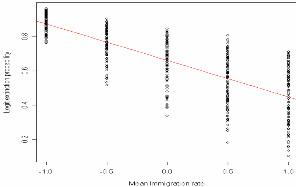
Figure 8a: Plot of logit extinction probability against standardized mean immigration rate, following sensitivity analysis. Linear fit gives adjusted r^2 = 0.61 .
