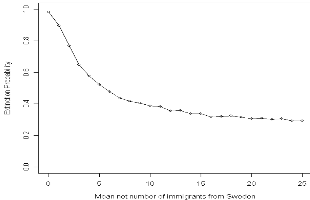
Figure 14: plot of extinction probability against mean number of immigrants, holding all other parameters constant.
