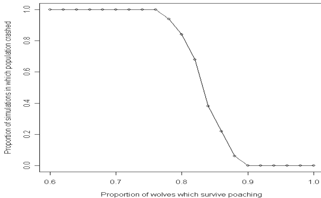
Figure 6: Plot of the proportion of simulations in which the wolf population had reached zero after 100 years (as proxy for extinction risk) against the proportion of wolves which survive poaching, for the entire Scandinavian population.
