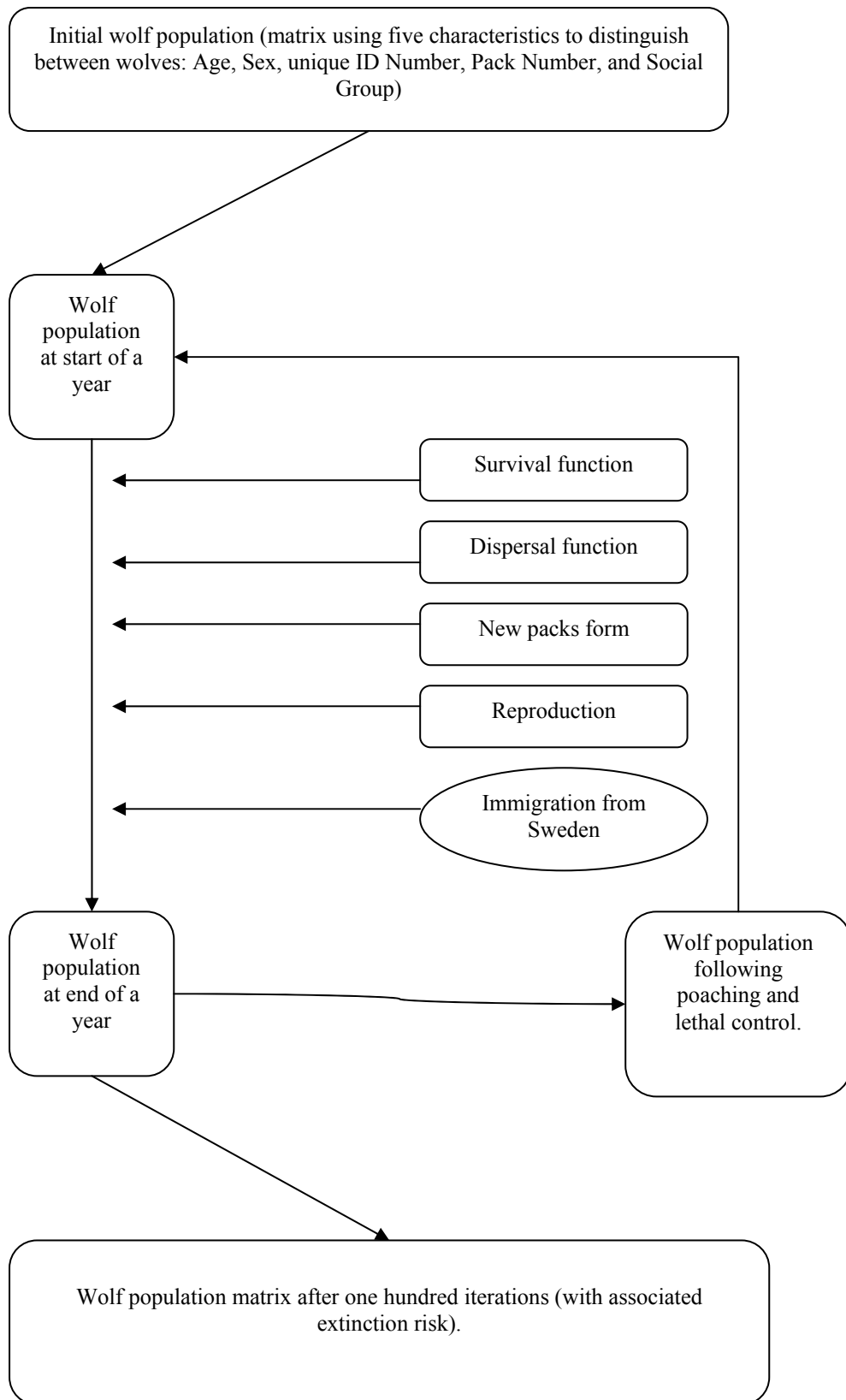
Figure 5: Flow diagram representing core aspect of model.
