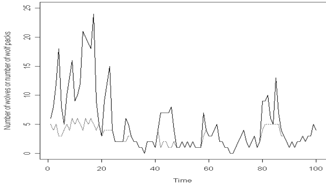
Figure 11: Example plot of wolf population and number of packs, in solid and dashed lines respectively, against time in years, with no culls, but poaching at present levels and with the preservation of the existing wolf zone. Extinction probability = 68 \pm 15\% .
