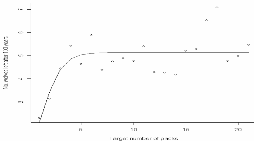
Figure 13: Plot of average number of wolves in population after 100 years (as proxy for inverse extinction risk) against target number of packs.
