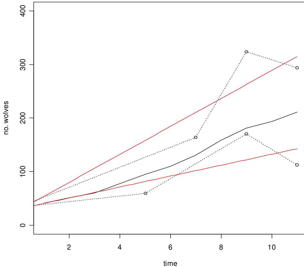
Figure 9: Plot of the number of wolves in Yellowstone Park, USA, against time in years, from 1995 onwards. Dotted lines represent the upper and lower bounds of empirical data for the region, straight lines represent the linear best fit for these data, and the solid curved line represents prediction of population trend made by the PVA model, using the empirical initial population and mortality rates.
