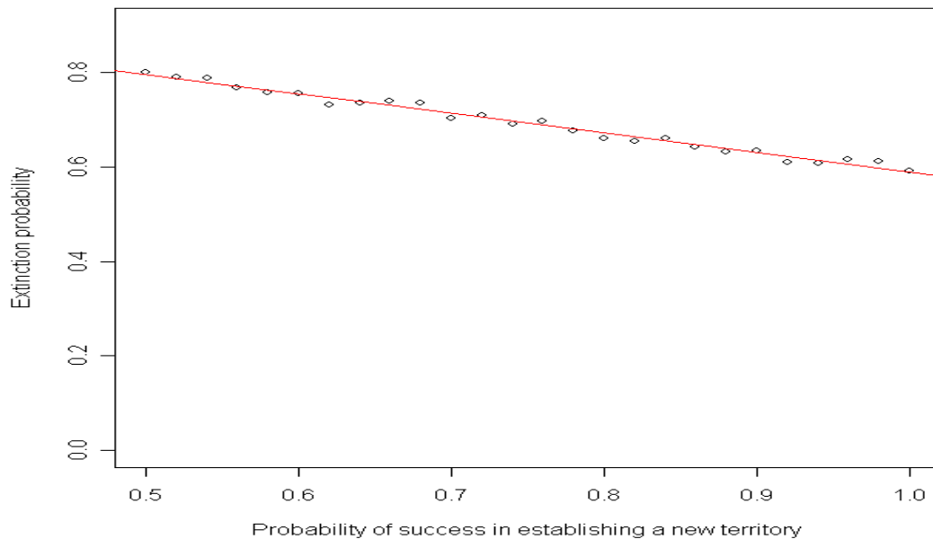
Figure 15: plot of extinction probability against probability of success in establishing territory, with linear line of best fit (adjusted r^2 = 0.98 )
