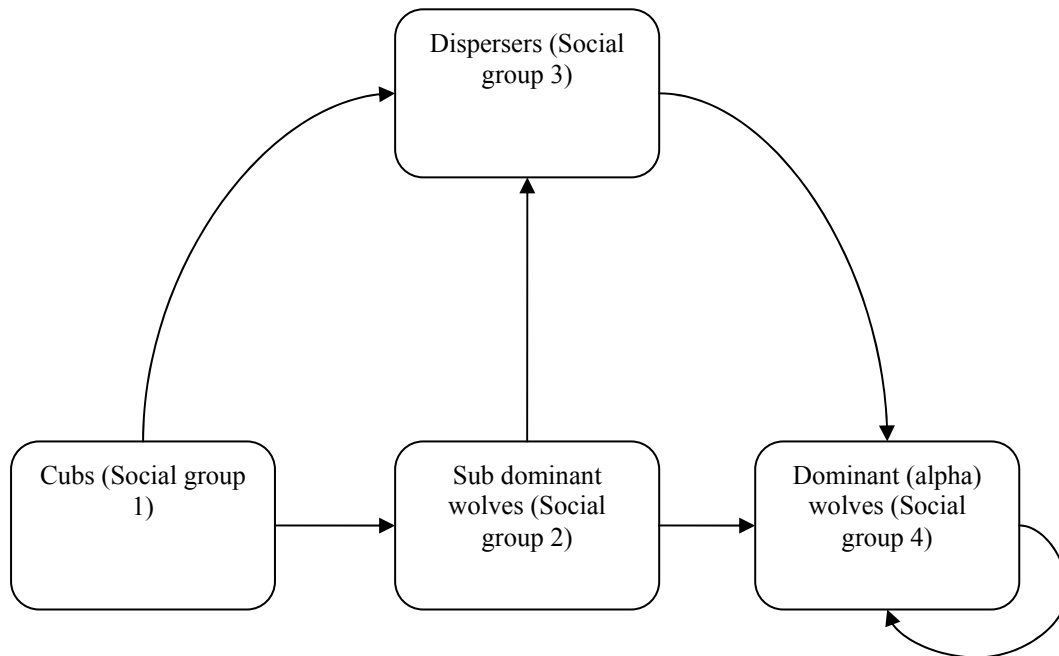
Figure 4: Flow diagram showing how the wolf social hierarchy was represented in the model using four social groups, and direction of transition between groups.
