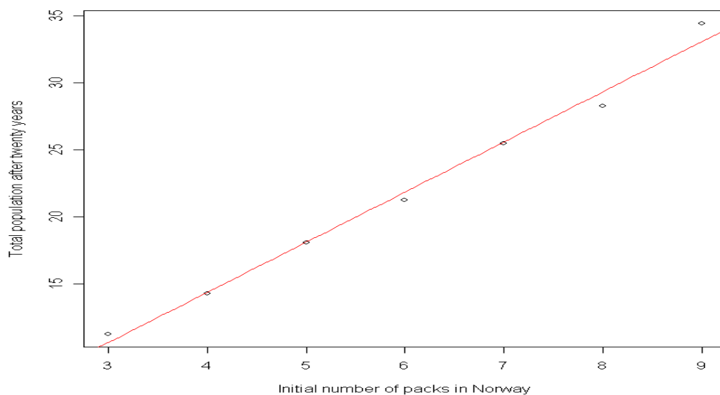
Figure 17: Plot of total population after twenty years, as proxy for success in re-establishing, against starting number of packs as reflective of the present regime. Line shown is linear best fit.
