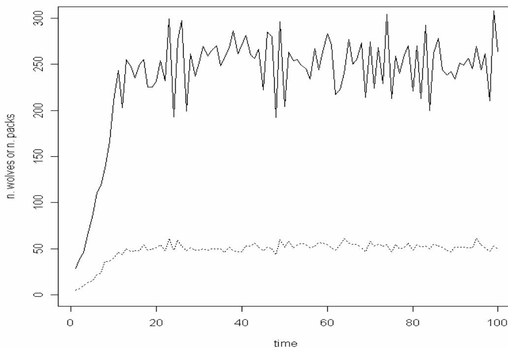
Figure 10: Example plot of wolf population and number of packs, in solid and dashed lines respectively, against time in years, with no anthropogenic intervention except the preservation of the existing wolf zone. Note that absolute values should not be given too much weight; this graph mainly demonstrates qualitative behaviour.
